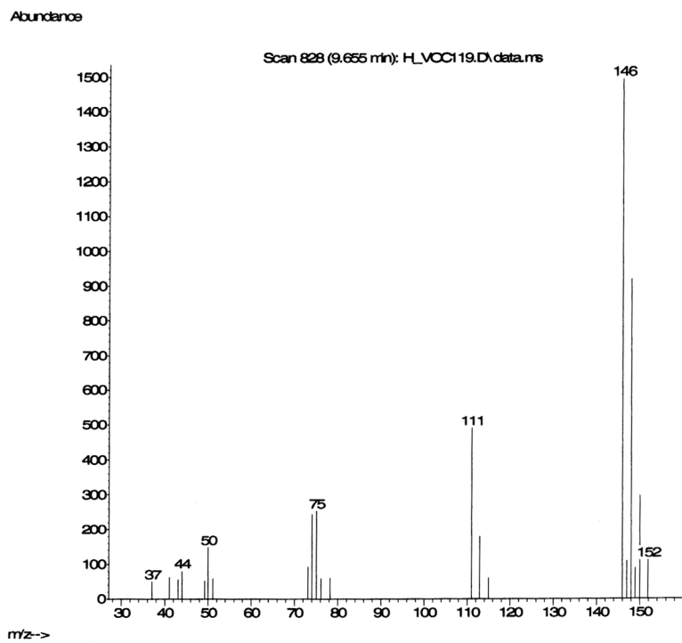
Figure 2: Electron impact mass spectra of p -DCB
