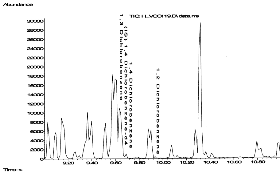
Figure 1: Total ion current (TIC) chromatogram of a honey extract spiked with 1, 2-DCB, 1, 4-DCB ( p -DCB), 1, 3-DCB d 4 - p -DCB
