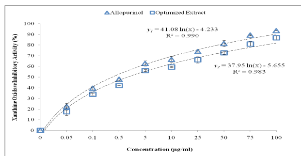
Figure 1. XO inhibitory activity (%) as a function of allopurinol and optimized extract concentrations. y_1 represents dose-response logarithmic function curve of allopurinol ( R^2 = 0.990 ) and y_2 represents dose-response logarithmic function curve of optimized extract ( R^2 = 0.983 ). Results are expressed as means \pm SD ( n = 3 ). IC_{50} value for allopurinol ( 3.74 \mu\text{g/ml} ) is lower than the optimized sample ( 4.33 \mu\text{g/ml} ).
